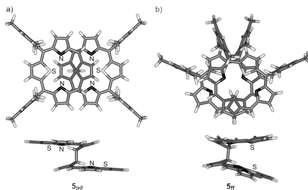
Figure 3. DFT-optimized structures of 5 : a) the parallel-displaced conformer ( 5 pd ) and b) the face-to-face skewed conformer ( 5 ff ). C(21)–C(21') bond lengths: a) 1.52 Å, b) 1.65 Å.
